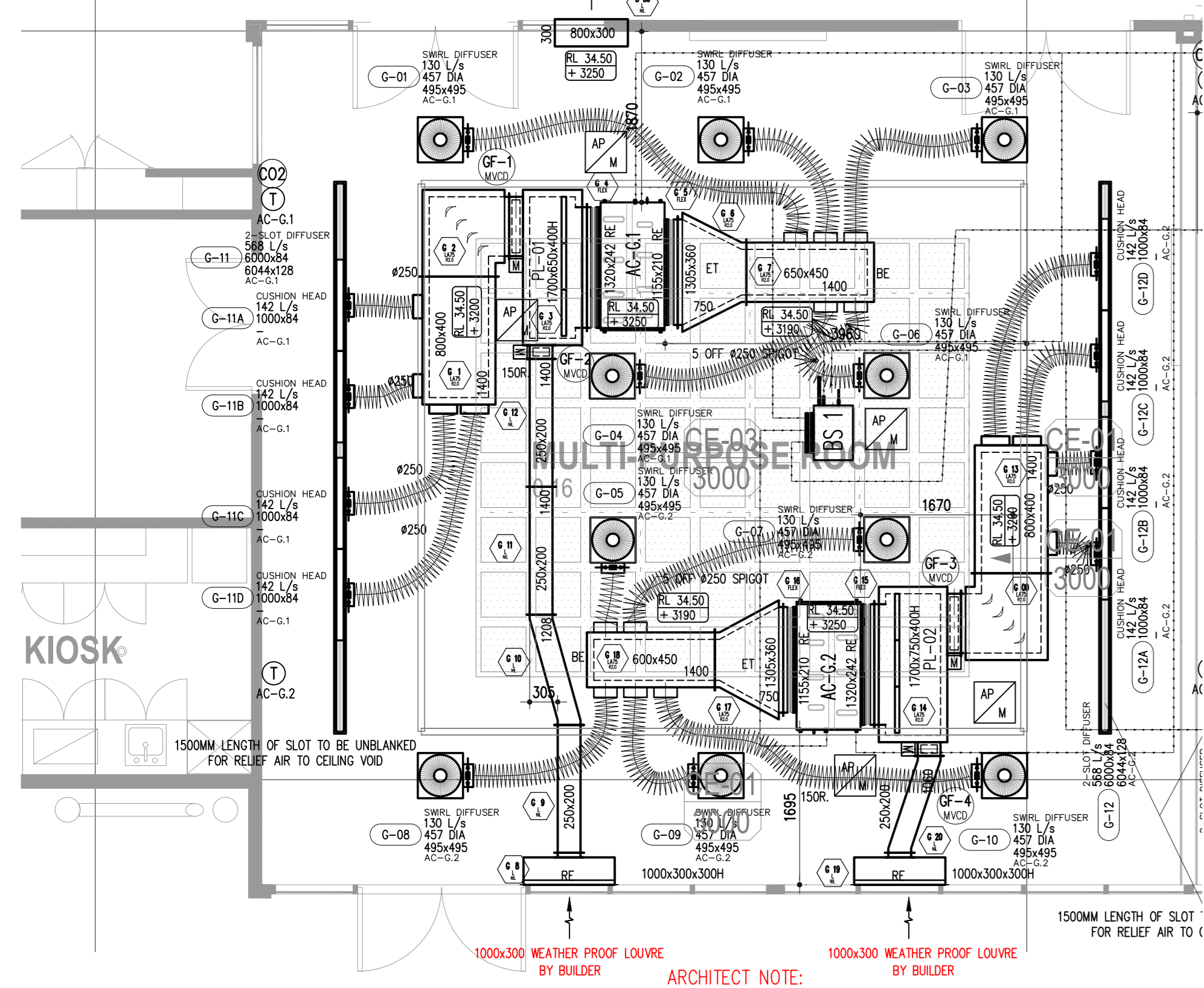
GROUND FLOOR - PART PLAN
