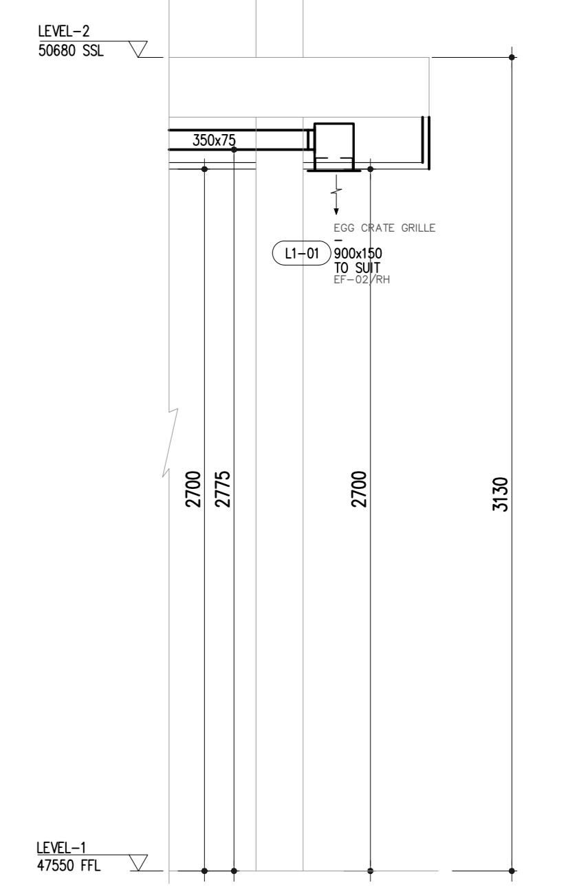
B TYP. SECTION DETAIL FOR SOFT GRILLE SCALE 1:20
