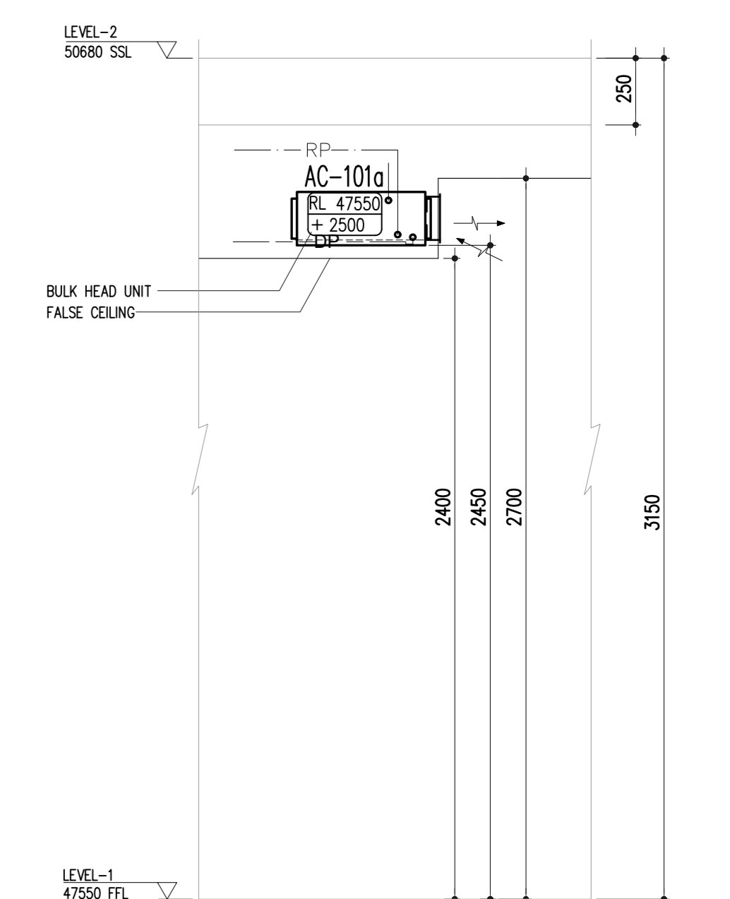
A TYP. SECTION OF BULKHEAD UNIT SCALE 1:20
